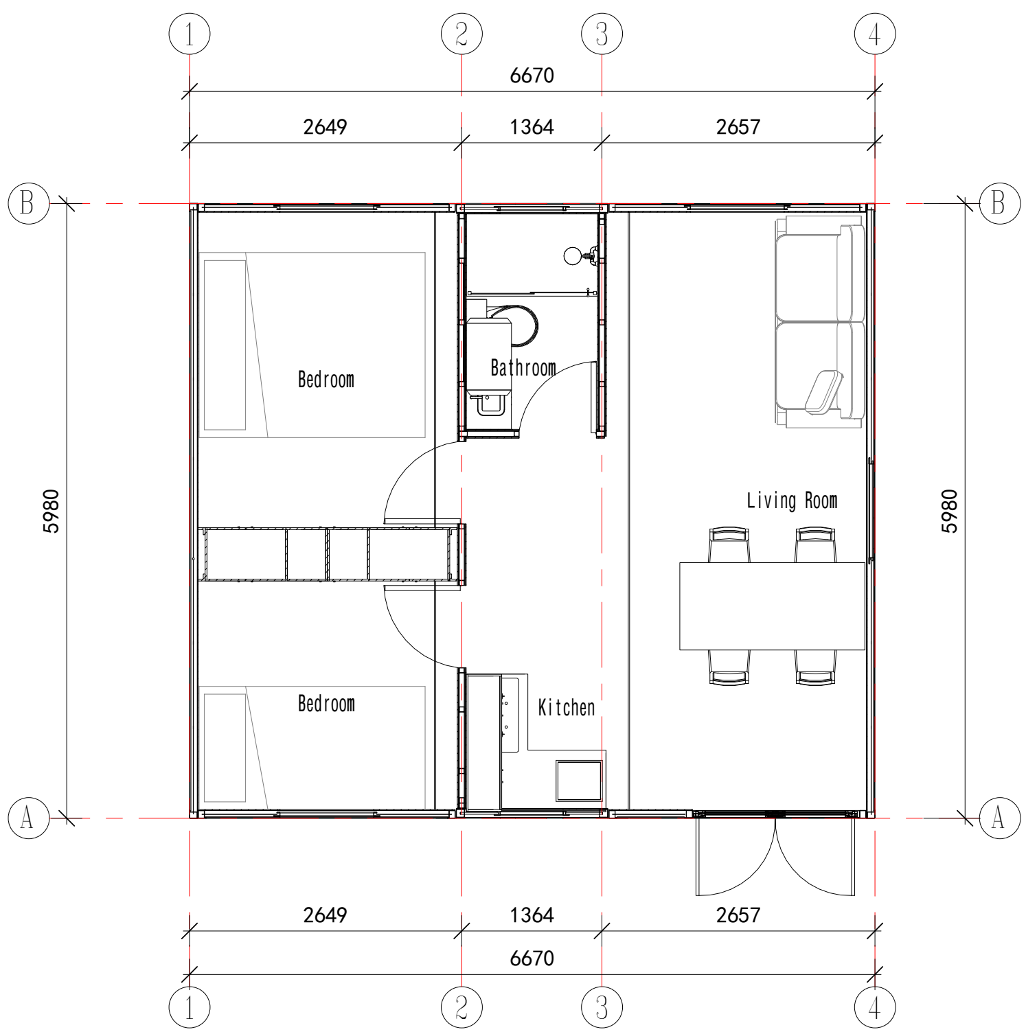
Floor Plan
